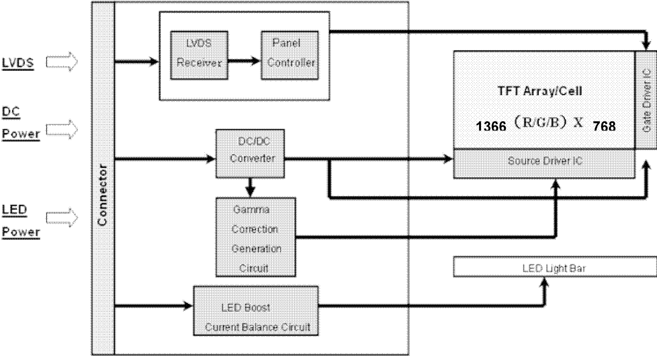
Figure 1 Block Diagram
