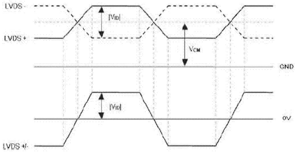
Figure 3 Voltage Definitions
