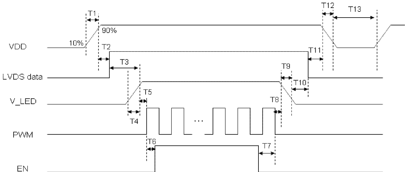
Figure 10 Power Sequence
