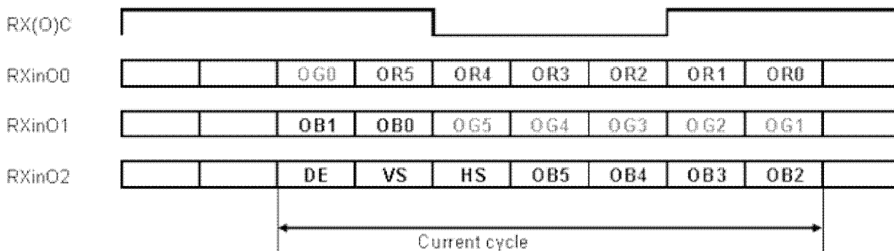
Figure 5 Data mapping
