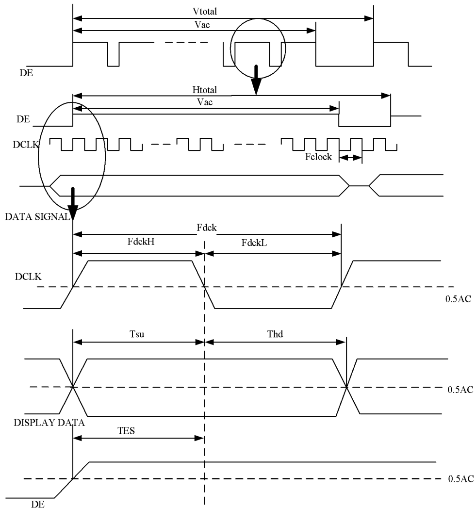
Figure 7 Timing Characteristics
