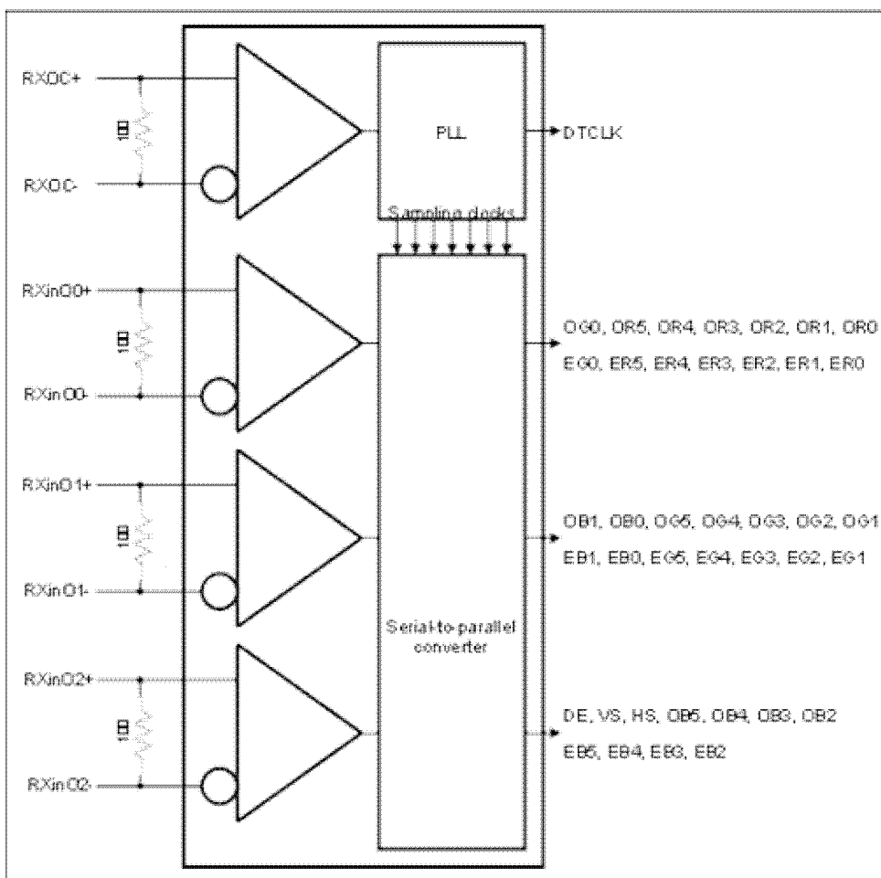
Figure 6 LVDS Receiver Internal Circuit
