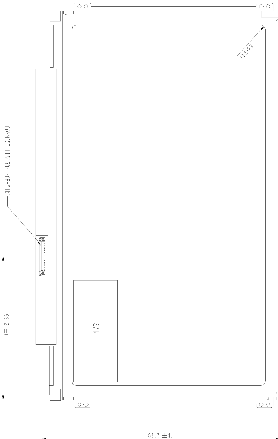
Figure 16 Reference Outline Drawing (Back Side)
