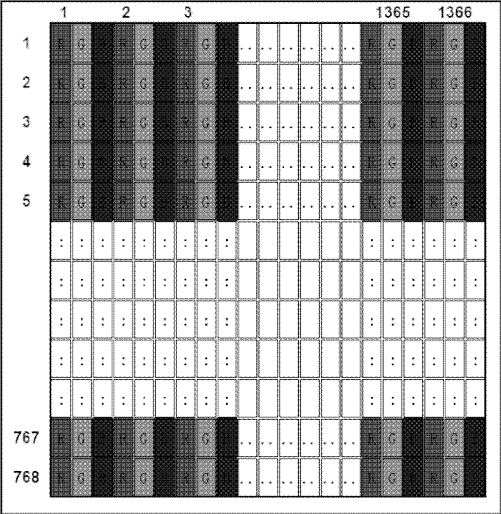
Figure 2 Pixel Format
